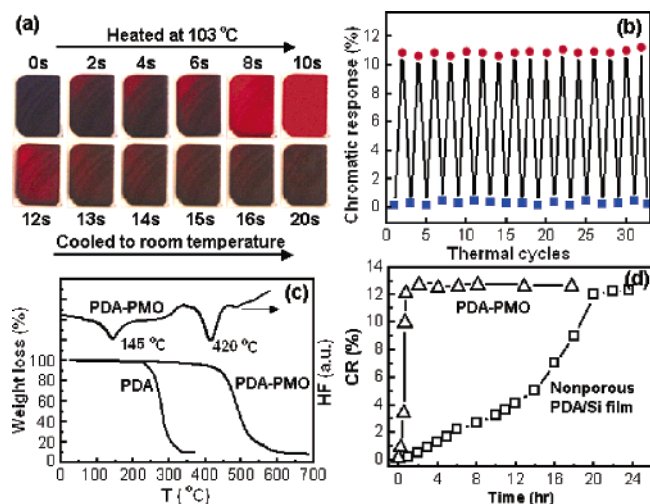
Figure 2. (a) Photographs of rapid thermochromic reversibility for the PDA-PMO nanocomposite film. (b) CR values of a PDA-PMO at 25 and 103 °C during thermal cycles. (c) DSC and TGA analysis of the PDA-PMO. TGA of the corresponding polydiacetylenic acid is also shown. (d) CR of the PDA-PMO before and after CTAB removal when exposed to a mixture of 10 M HCl and methanol (v/v = 7/1).
