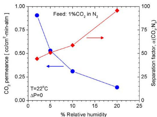
Fig. 7. Effect of relative humidity on CO 2 permeance and binary separation factor \alpha(\text{CO}_2:\text{N}_2) for a APTES:TEOS-derived aminosilicate membrane (ratio of -\text{NH}_2:\text{Si}=0.2 ). Feed is 1 vol.% CO 2 -balance N 2 . Operation in the Wicke–Kallenbach mode under \Delta P=0 .
