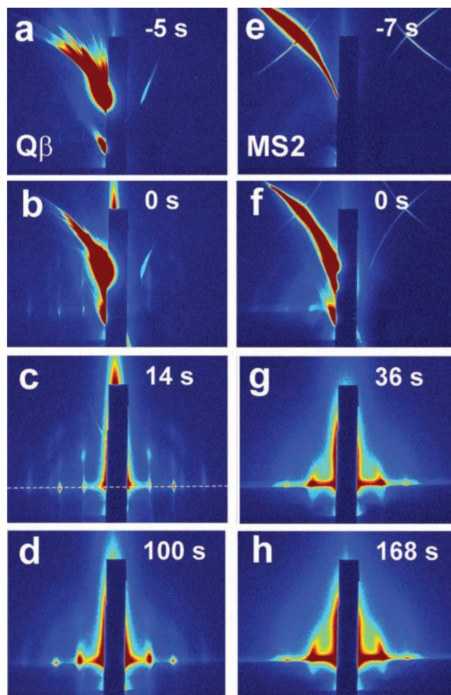
Figure 3. Time sequence of GISAXS data, referenced to the first emergence of the X-ray beam from behind the plate of the convective coater (a,e), comparing the self-assembly of Q \beta (a–d) and MS2 (e–h) from deionized (DI) water under identical coating conditions. For Q \beta , assembly of 2D arrays occurs without intermediate aggregation or structure formation (b,c); weakened and broader (20) and (21) reflections indicate loss of long-range order during the final stage of film drying (d). MS2 assembly is characterized by poor long-range order in comparison to Q \beta (g), including the formation of a glassy multilayer film upon H 2 O evaporation (h) and a much smaller domain size. Plate movement is from left to right in both series of images.
