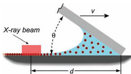
Figure 1. Schematic of the convective assembly process used in GISAXS studies of VLP self-assembly. A plate at angle \theta is moved across a substrate at velocity v , entraining a meniscus from which a particle film is deposited. The self-assembly process is probed at a fixed position on the substrate denoted by the shaded area; d is the time-dependent distance between the X-ray beam and the edge of the coater.
