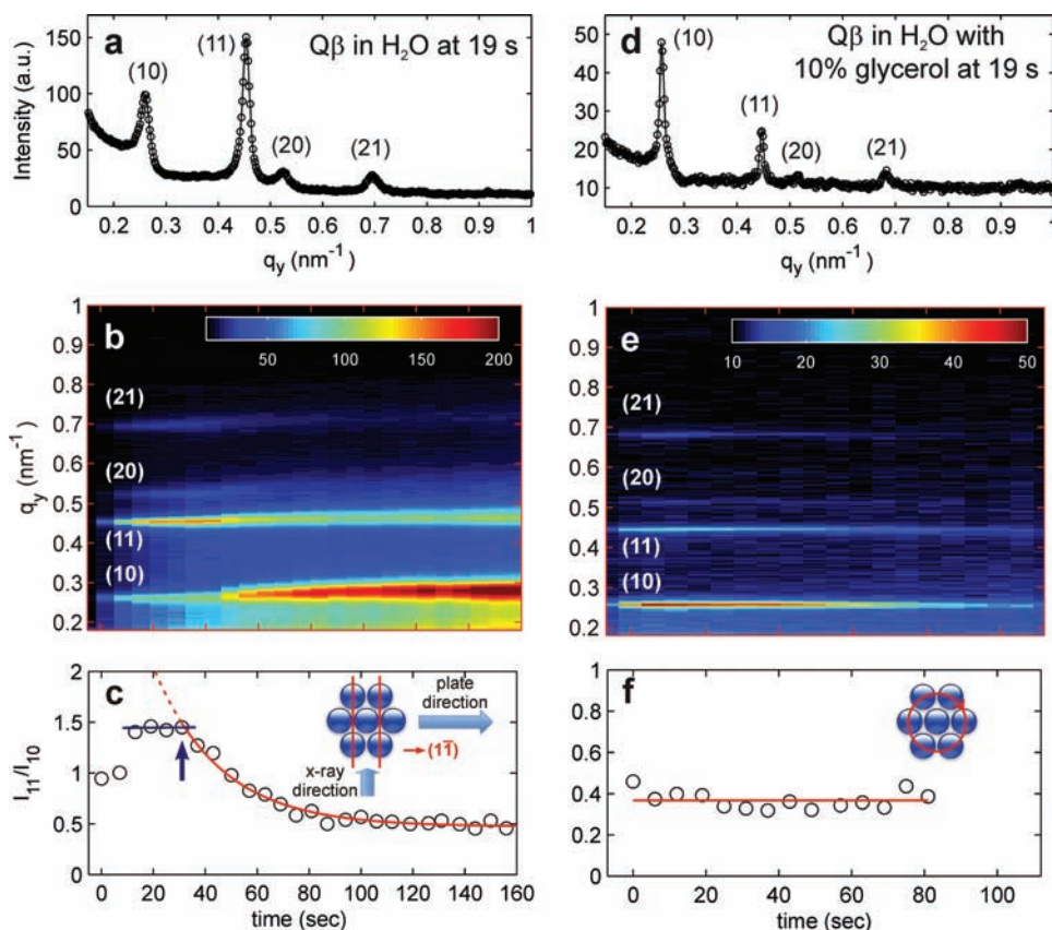
Figure 4. a) A horizontal linecut at q_z = 0.24 \pm 0.02 \text{ nm}^{-1} taken from the GISAXS data for Q\beta self-assembled in DI water at t = 19 \text{ s} (the dashed line marked in Figure 3c). The first four Bragg diffractions are indexed to 2D hexagonal packing. b) The time evolution of this horizontal linecut. c) The ratio of the integrated intensities underneath the (11) and (10) reflections, after background subtraction. The red line is a fit to an exponential decay function as described in the text, and the inset represents the dominant 2D domain orientation induced by convective transport. d–f) The corresponding panels from GISAXS for Q\beta in water with 10% glycerol.
