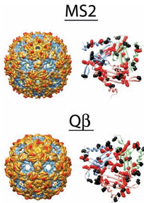
Figure 2. Structures of Q \beta and MS2 bacteriophages (left), and close-ups of phage subunit structure for Q \beta and MS2 (right), with acidic and basic amino acid residues highlighted in red and black, respectively.
